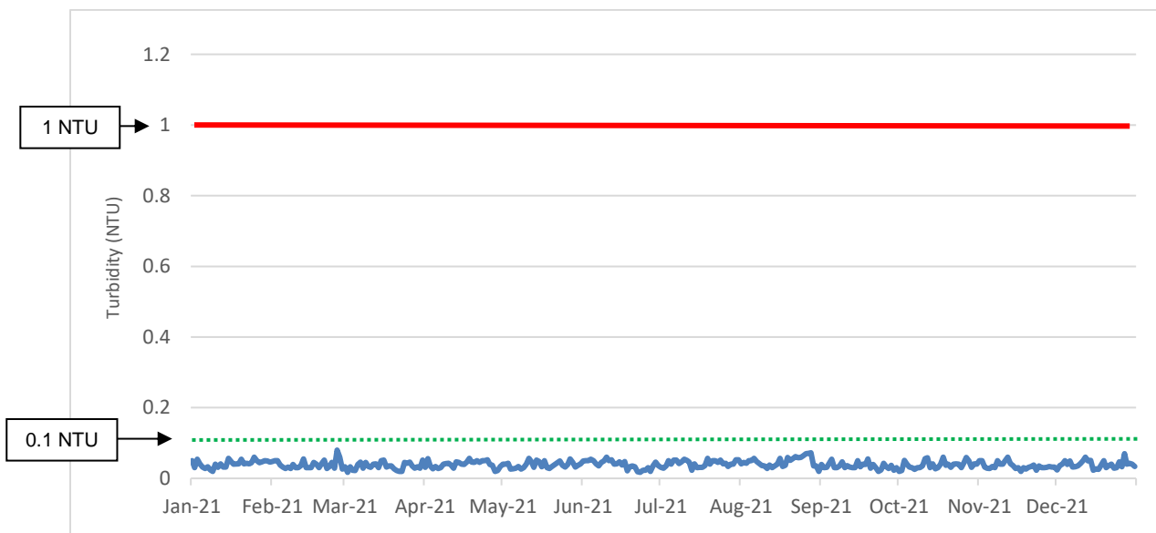
Graph 1 – potable water turbidity at the SFWTP
