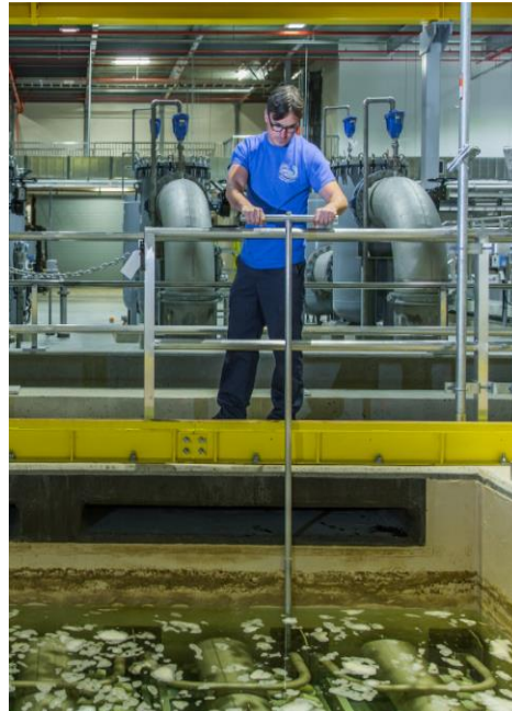
South Fork Water Treatment Plant – primary membrane maintenance
